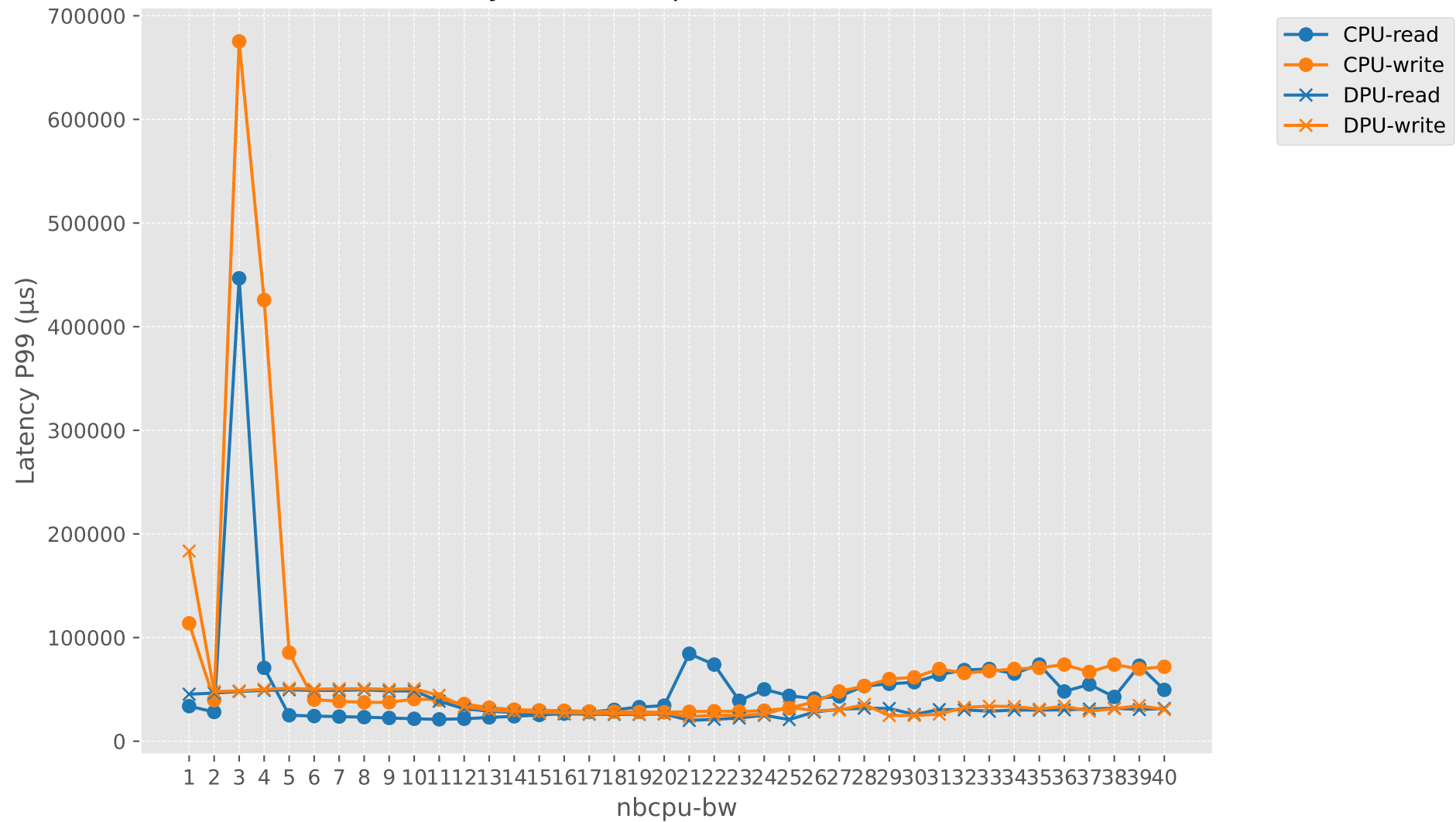
Latency P99 vs nbcpu-bw (CPU vs DPU)
